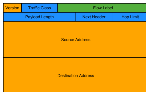
IPv6-header
