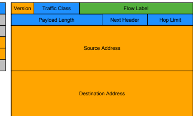
IPv6-header
