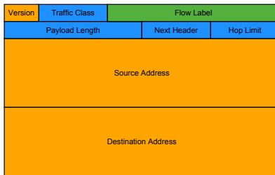
IPv6-header
